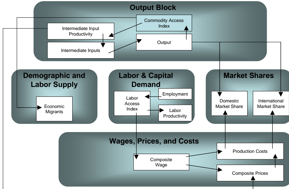
Figure A.2: REMI Policy Insight Geography Linkages
