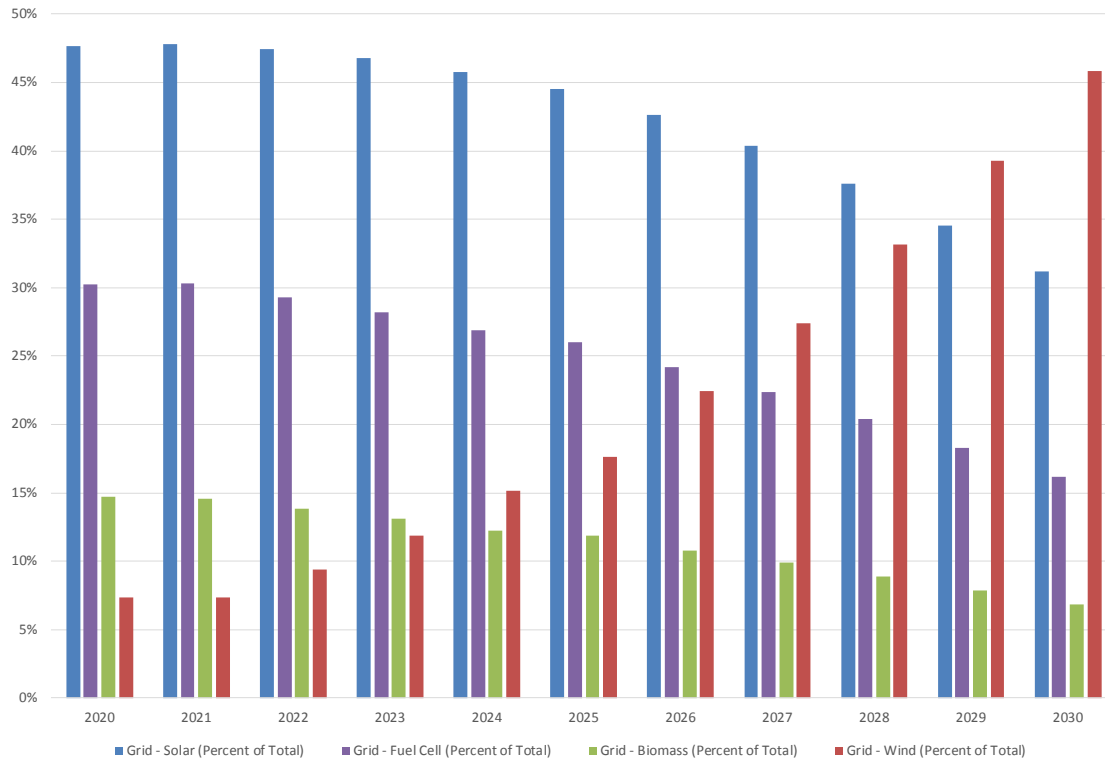
Figure 25: Grid-Scale Generation Added as a Percent of Total GWh Added
