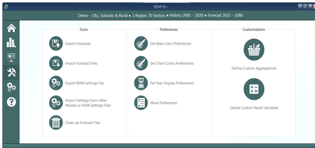
Figure 32: Tools & Settings
