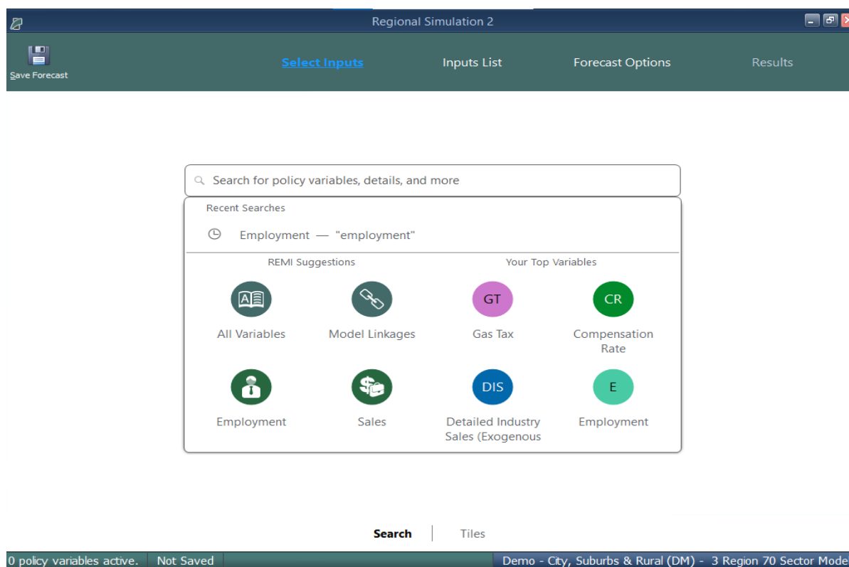
Figure 52: Forecast Window
