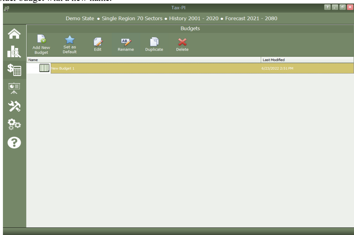
Figure 6: Budget List
