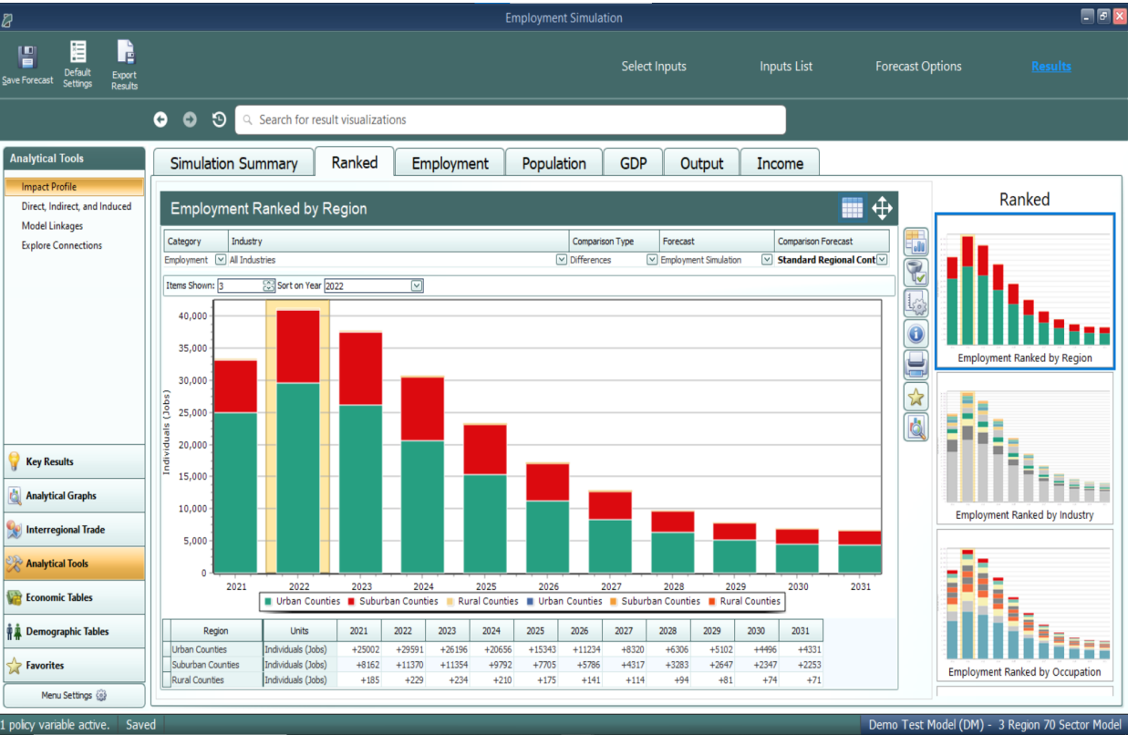
Figure 85: Ranked Visualizations
