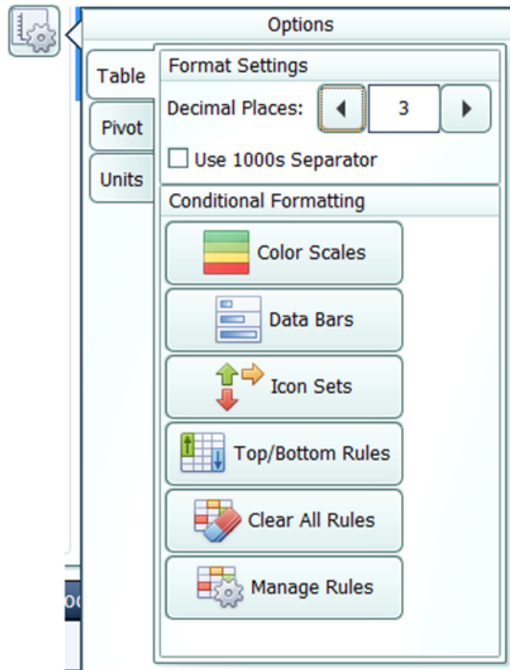
Figure 84: Conditional Formatting
