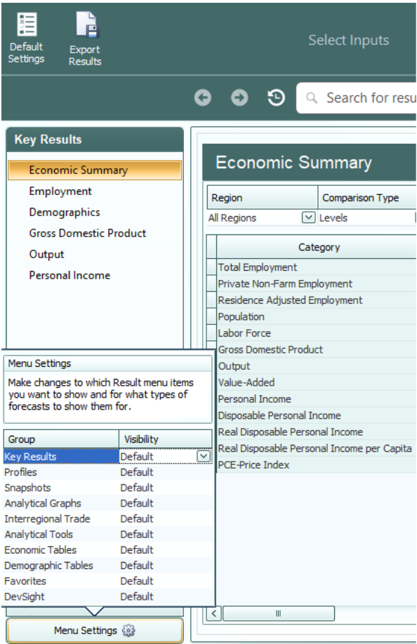
Figure 79: Menu Settings
