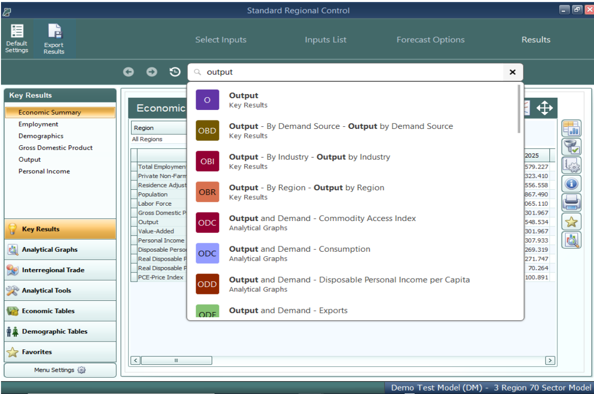
Figure 83: Results Search
