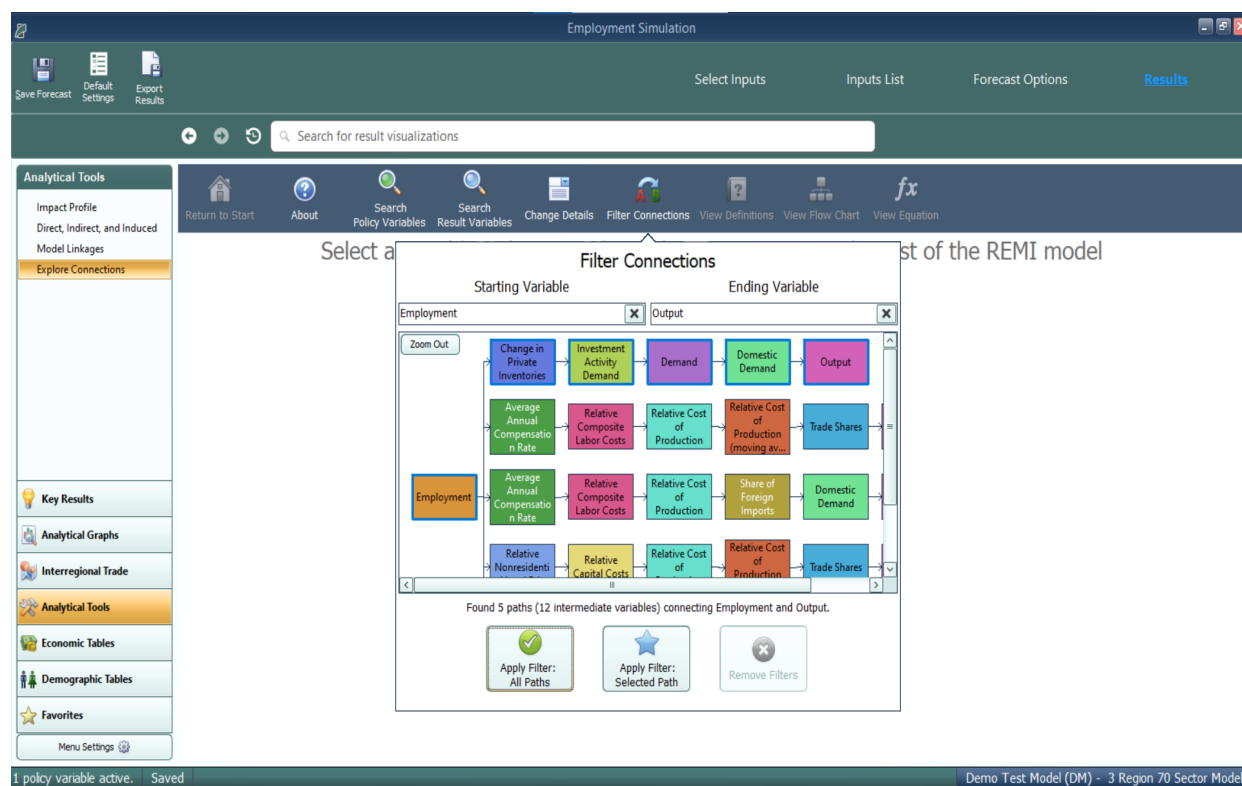
Figure 93: Connections Filter
